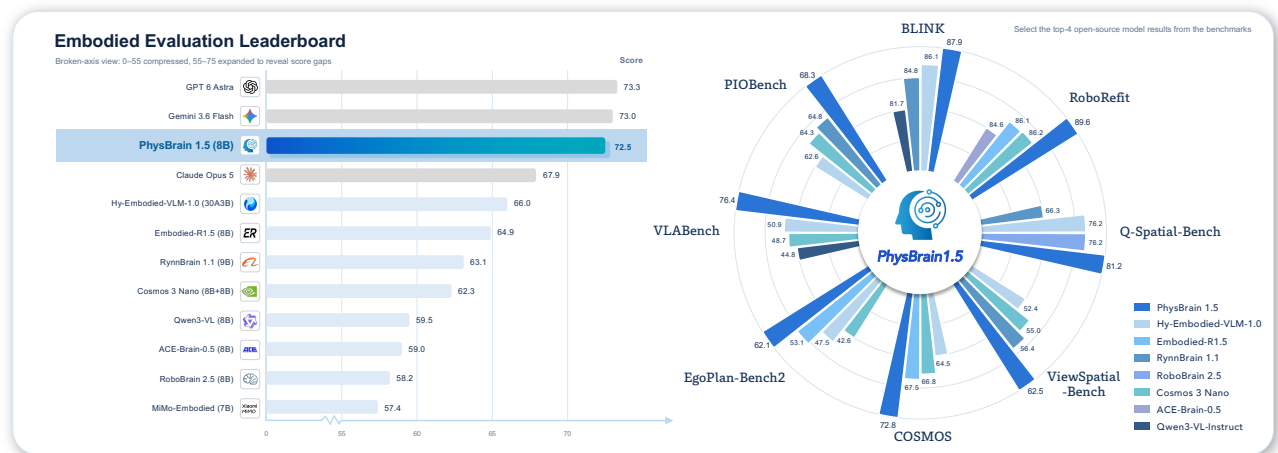
Figure 1 Leading overall performance on the report’s embodied benchmark suite. PhysBrain 1.5 achieves an overall score of 72.5 with 8B parameters, ranking first among all open-sourced models and delivering performance on par with leading proprietary systems.
